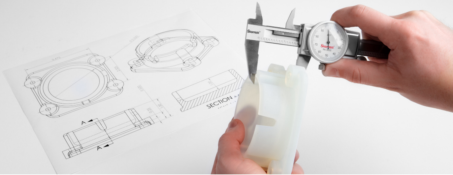
Inspecting a 3D printed part with a caliper to verify dimensional accuracy.
