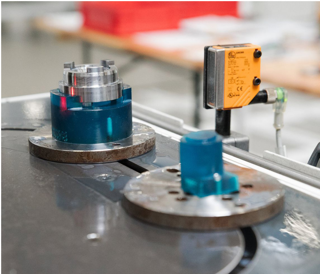
3D printed jigs in an automated production line at Pankl Racing Systems.
