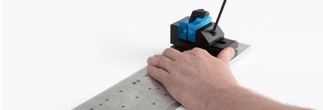
A part being clamped between soft jaw inserts, printed in Formlabs Tough Resin.
